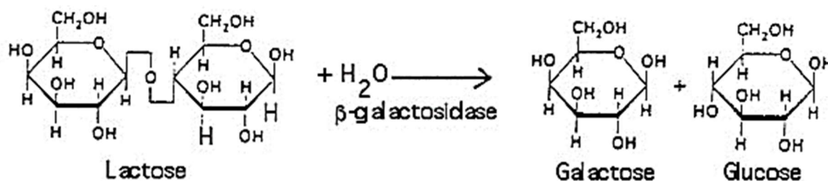
Figure 1: Enzymatic conversion of lactose operated by \beta -galactosidase in milk ( https://openwetware.org/wiki/BISC220/S11:_Mod_1_Lab_1 ).
