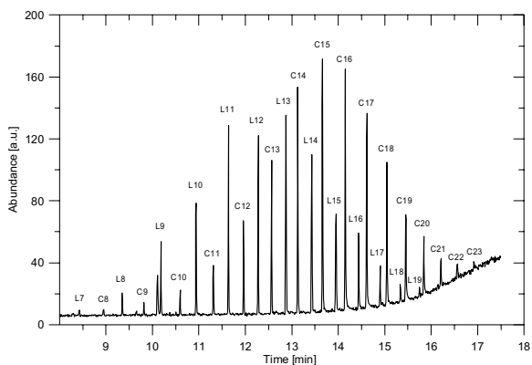
Figure 5 GC-MS of residue of sample B at the third one hour exposition at 175 °C
